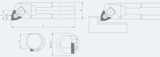
TEKNİK ÇİZİM / TECHNICAL DRAWING
