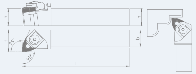
TEKNİK ÇİZİM / TECHNICAL DRAWING
