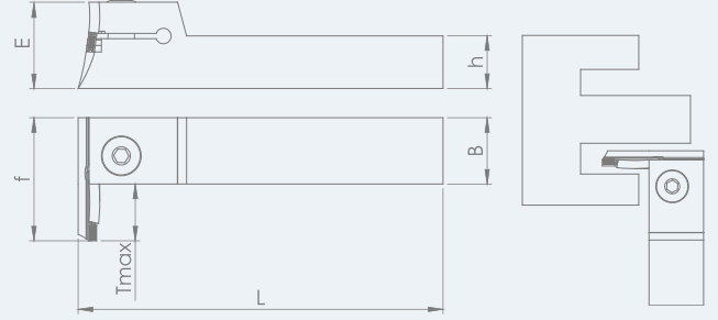
TEKNİK ÇİZİM / TECHNICAL DRAWING
