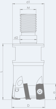
TEKNİK ÇİZİM / TECHNICAL DRAWING
