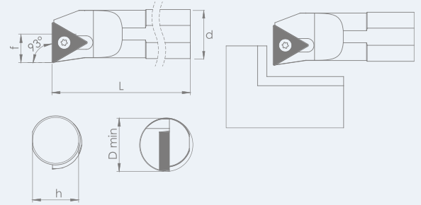
TEKNİK ÇİZİM / TECHNICAL DRAWING
