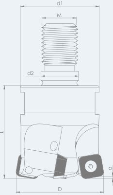
TEKNİK ÇİZİM / TECHNICAL DRAWING
