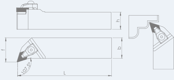
TEKNİK ÇİZİM / TECHNICAL DRAWING
