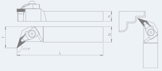
TEKNİK ÇİZİM / TECHNICAL DRAWING
