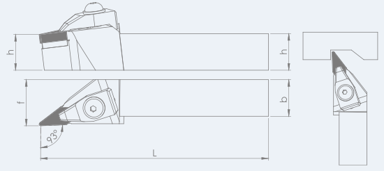
TEKNİK ÇİZİM / TECHNICAL DRAWING
