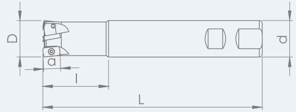
TEKNİK ÇİZİM / TECHNICAL DRAWING
