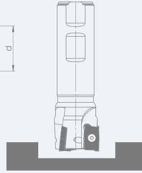
TEKNİK ÇİZİM / TECHNICAL DRAWING
