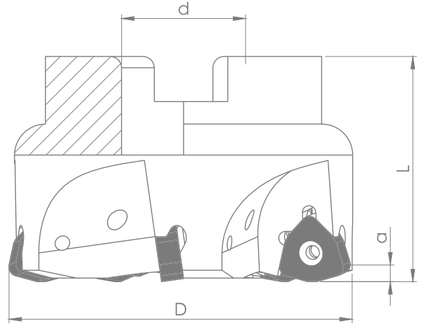
TEKNİK ÇİZİM / TECHNICAL DRAWING
