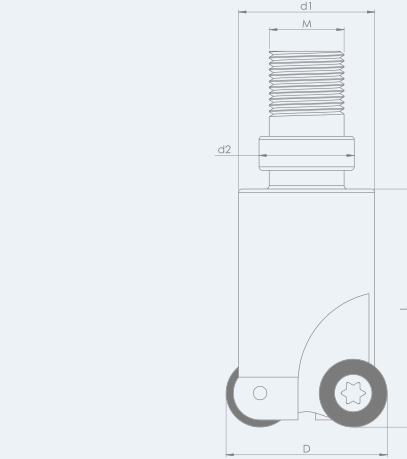
TEKNİK ÇİZİM / TECHNICAL DRAWING
