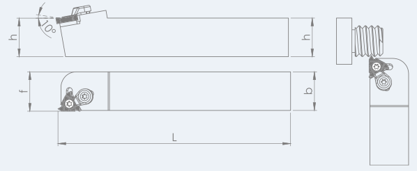
TEKNİK ÇİZİM / TECHNICAL DRAWING
