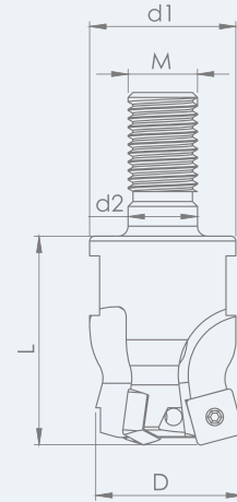
TEKNİK ÇİZİM / TECHNICAL DRAWING
