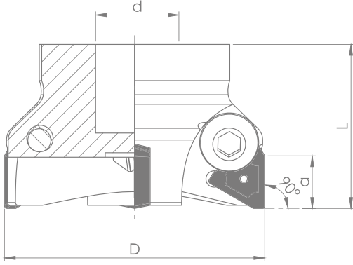
TEKNİK ÇİZİM / TECHNICAL DRAWING
