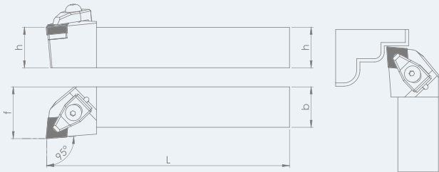
TEKNİK ÇİZİM / TECHNICAL DRAWING
