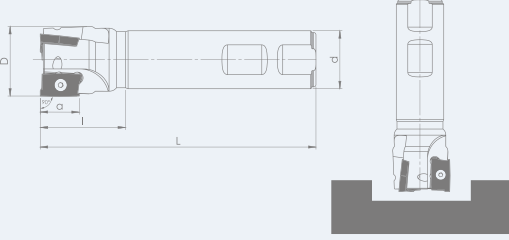
TEKNİK ÇİZİM / TECHNICAL DRAWING
